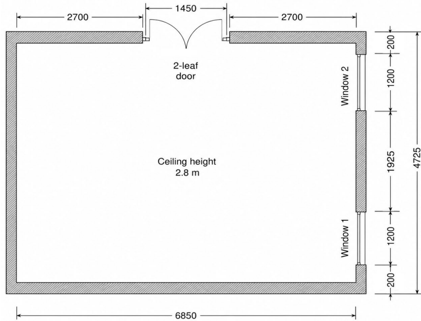
INITIAL FLOOR PLAN
